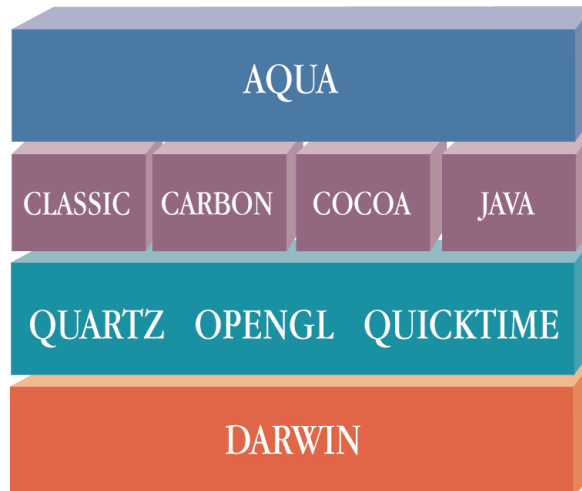
Mac OS X system architecture
