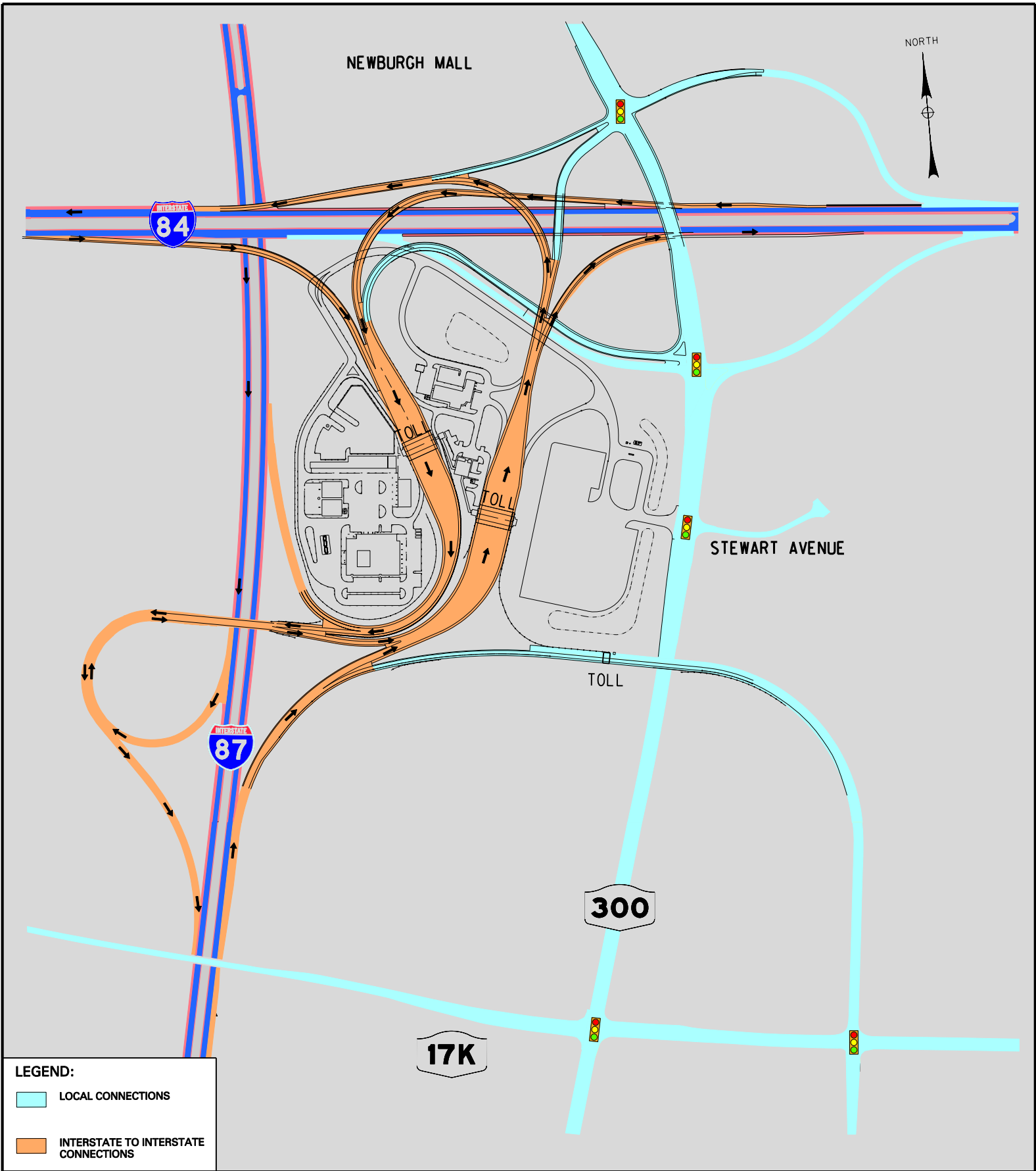
RECONSTRUCTED INTERCHANGE
