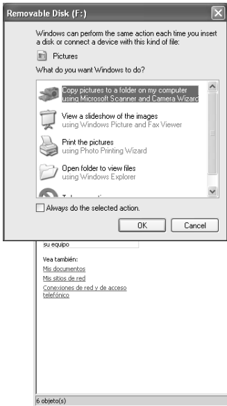
Windows XP
